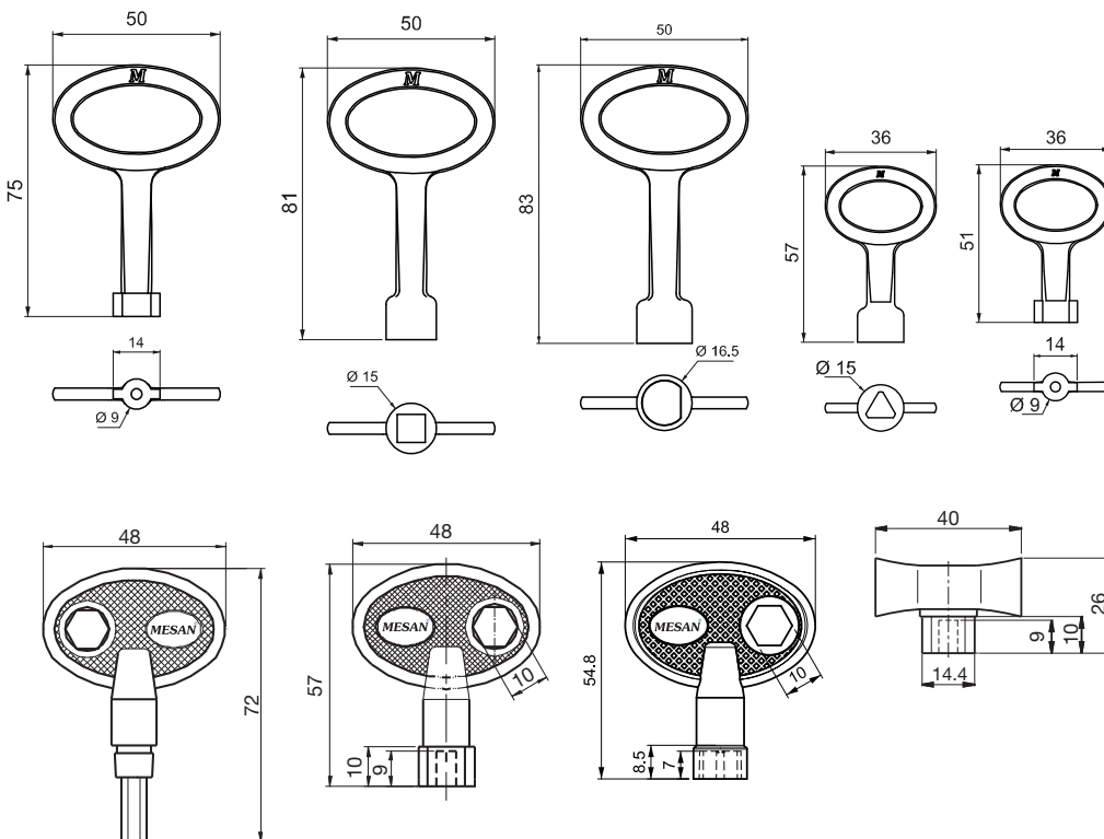
Outer dimensions
